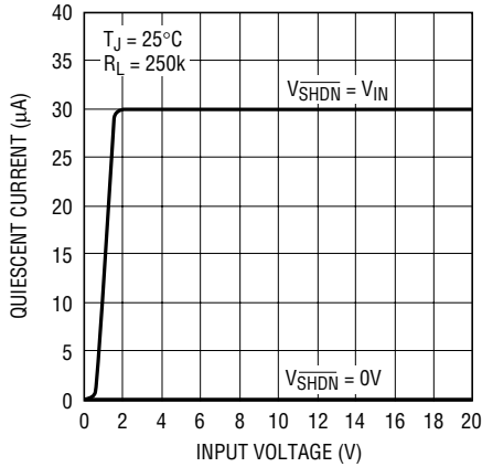
LT1763 Quiescent Current
