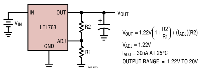
Figure 2. Adjustable Operation
