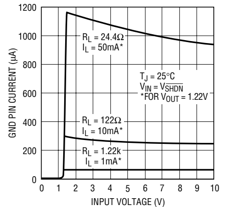
LT1763 GND Pin Current
