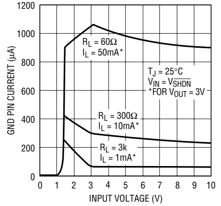
LT1763-3 GND Pin Current
