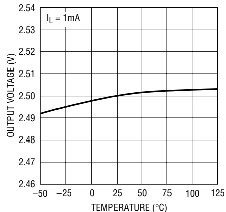
LT1763-2.5 Output Voltage
