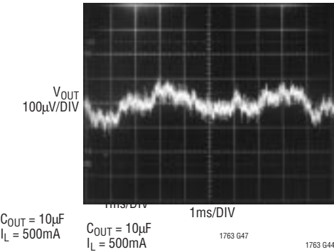
LT1763-5 10Hz to 100kHz Output Noise C_{BYP} = 1000pF
