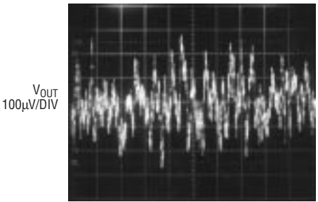
LT1763-5 10Hz to 100kHz Output Noise C_{BYP} = 100pF
